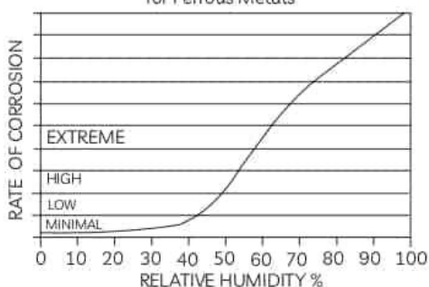
Typical Rate of Corrosion for Ferrous Metals
