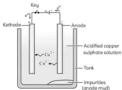
Fig. 6 Electrolytic refining of copper
