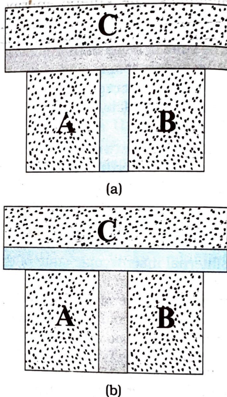
Fig. 12.2 (a) Systems A and B are separated by an adiabatic wall, while each is in contact with a third system C via a conducting wall. (b) The adiabatic wall between A and B is replaced by a conducting wall, while C is insulated from A and B by an adiabatic wall.
