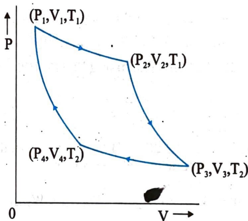
Fig. 12.11 Carnot cycle for a heat engine with an ideal gas as the working substance.
