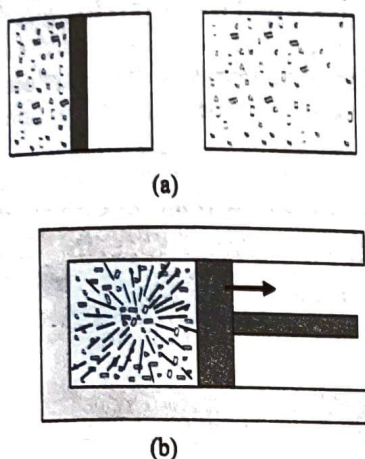
Fig. 12.6 (a) The partition in the box is suddenly removed leading to free expansion of the gas. (b) A mixture of gases undergoing an explosive chemical reaction. In both situations, the gas is not in equilibrium and cannot be described by state variables.
