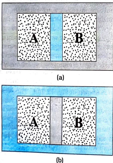
Fig. 12.1 (a) Systems A and B (two gases) separated by an adiabatic wall - an insulating wall that does not allow flow of heat. (b) The same systems A and B separated by a diathermic wall - a conducting wall that allows heat to flow from one to another. In this case, thermal equilibrium is attained in due course.
