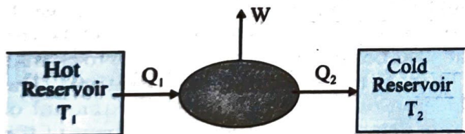
Fig. 12.9 Schematic representation of a heat engine. The engine takes heat Q_1 from a hot reservoir at temperature T_1 , releases heat Q_2 to a cold reservoir at temperature T_2 and delivers work W to the surroundings.
