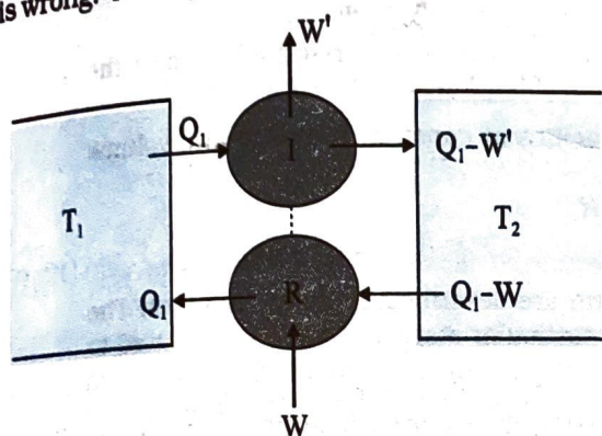
Fig. 12.12 An irreversible engine (I) coupled to a reversible refrigerator (R). If W' > W , this would amount to extraction of heat W' - W from the sink and its full conversion to work, in contradiction with the Second Law of Thermodynamics.
