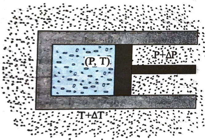
Fig. 12.7 In a quasi-static process, the temperature of the surrounding reservoir and the external pressure differ only infinitesimally from the temperature and pressure of the system.
