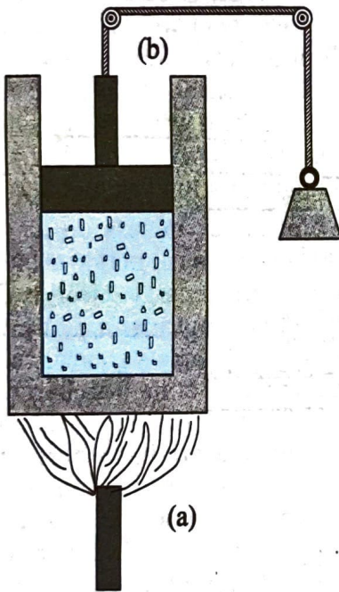
Fig. 12.4 Heat and work are two distinct modes of energy transfer to a system that results in change in its internal energy. (a) Heat is energy transfer due to temperature difference between the system and the surroundings. (b) Work is energy transfer brought about by means (e.g. moving the piston by raising or lowering some weight connected to it) that do not involve such a temperature difference.
