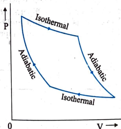
Fig. 12.8 P - V curves for isothermal and adiabatic processes of an ideal gas.
