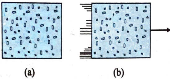
Fig. 12.3 (a) Internal energy U of a gas is the sum of the kinetic and potential energies of its molecules when the box is at rest. Kinetic energy due to various types of motion (translational, rotational, vibrational) is to be included in U . (b) If the same box is moving as a whole with some velocity, the kinetic energy of the box is not to be included in U .
